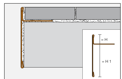
Schlüter®-SCHIENE-STEP-EB
